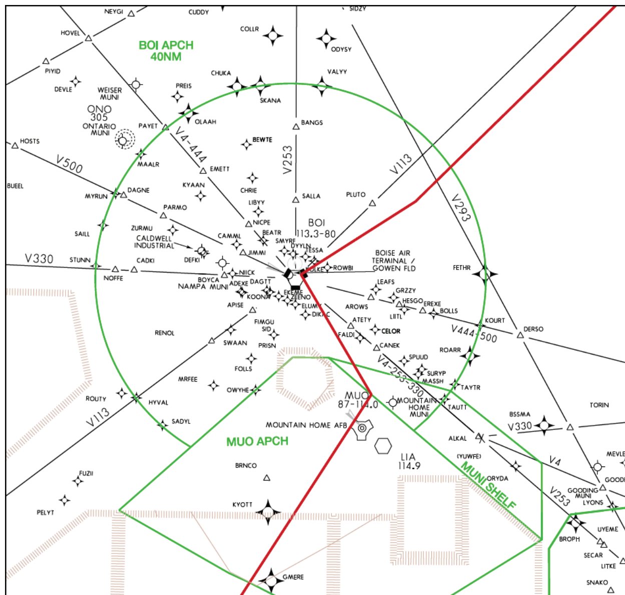
Figure 1. Big Sky TRACON Lateral Airspace Depiction
