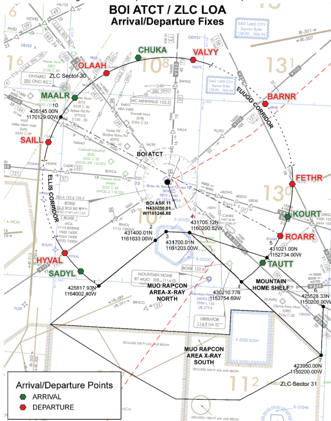
Figure 1. Arrival/Departure Fixes and Corridors Depiction
